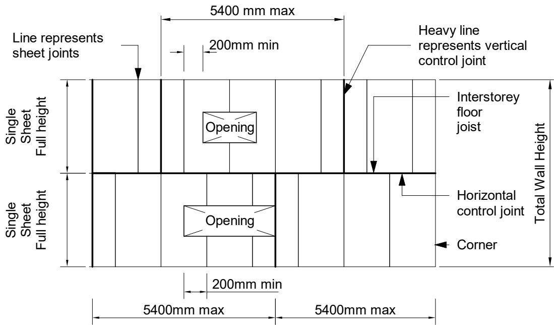
Typical Two Story Control Joint Layout
