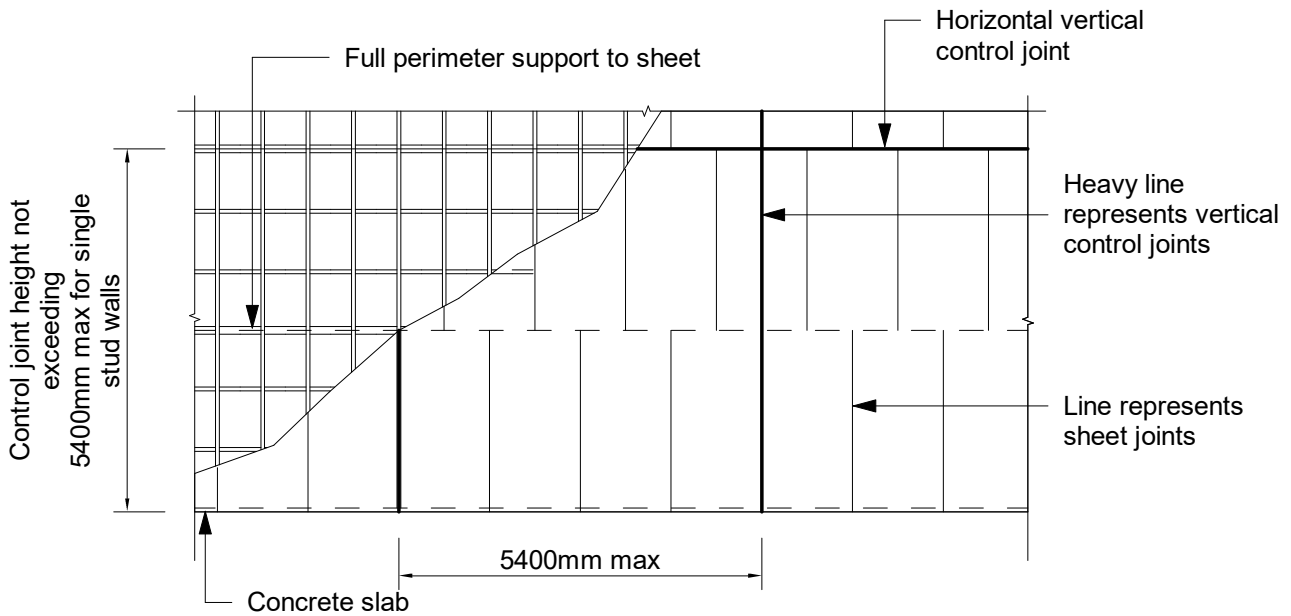
Typical High Stud Wall Control Joint Layout
