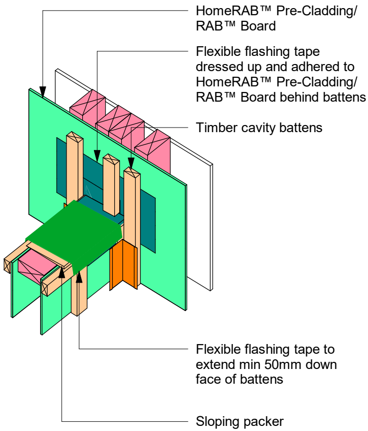
Flashing Tape Application Prior to Batten and Metal Flashing Fixing
