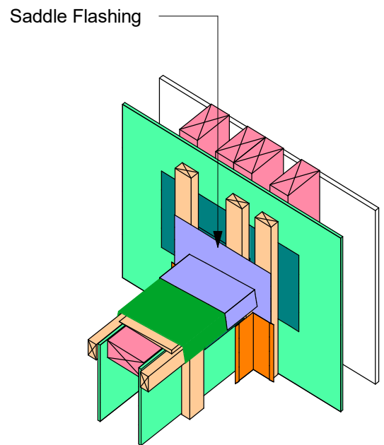
Saddle Flashing Application Prior to Cladding and Cap Flashing Fixing
