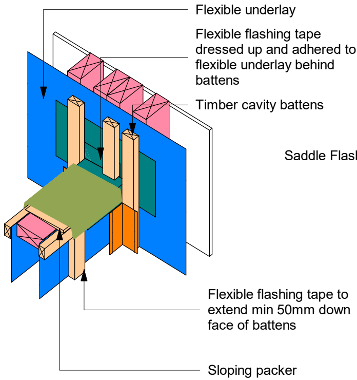
Batten and Flashing Tape Application Prior to Metal Flashing Fixing
